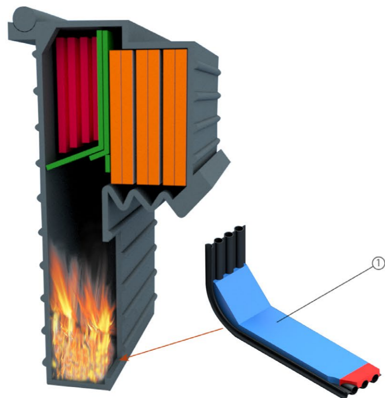
Recovery Boiler
