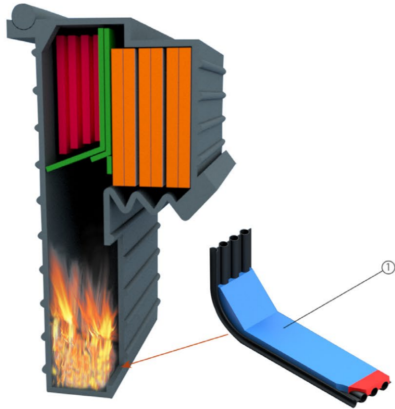
Recovery Boiler
